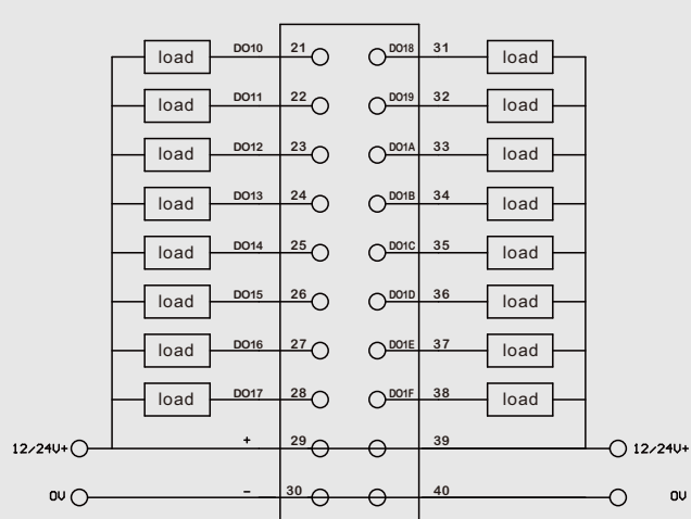
17~32-CH NPN TYPE DO OUTPUT
