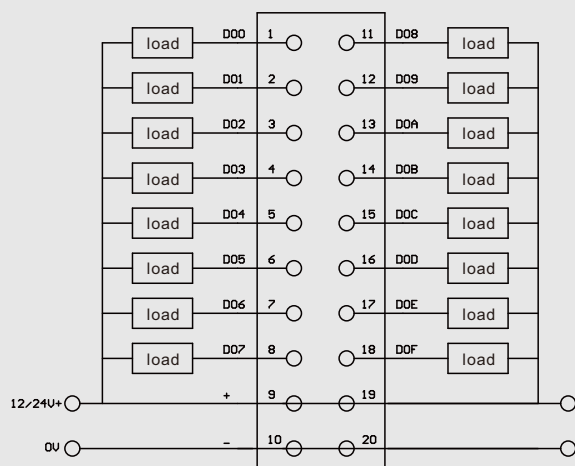
1~16-CH NPN TYPE DO OUTPUT
